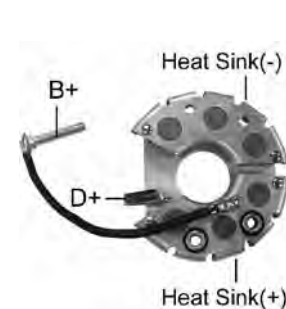
RB-137H *M6 Battery Post *6-35A Amp Diodes Replaces BOSCH : 9-121-080-595 Unit No. BOSCH : 9-120-080-041, 9-120-080-061...
