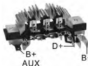
RT-05H *6-35 Amp Diodes
