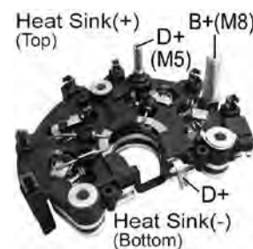
RB-134H *M5 Battery Post *6-50A Avalanche Diode
