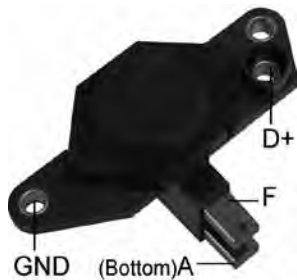
VR-VW009 *Voltage Set Point:14.5V
