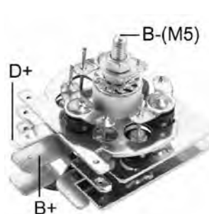
RL-13H *M5 Battery Post *9-35 Amp Diodes
