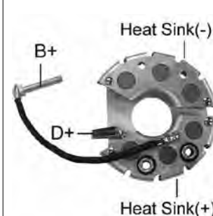
RB-137HV Same as RB-137H but W/6-50 Amp Diodes *M6 Battery Post Replaces BOSCH : 9-121-080-595 Unit No. BOSCH : 9-120-080-041, 9-120-080-061 ...
