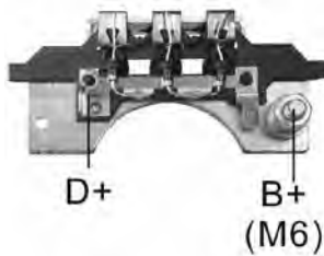
RT-01H *6-35 Amp Diodes
