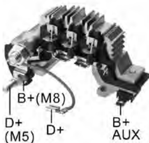
RT-10H *6-35 Amp Diodes *Economy Version: RT-10HA
