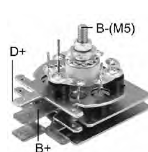
RL-13 *9-25 Amp Diodes
