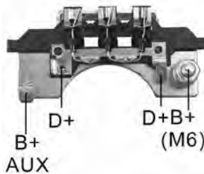
RT-03H *6-35 Amp Diodes
