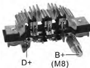
RT-04H *6-35 Amp Diodes
