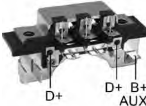
RT-02H *6-35 Amp Diodes
